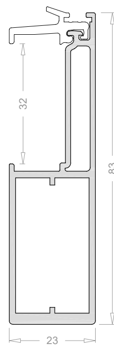
Hoja cruce ref. 23 mm 3619
