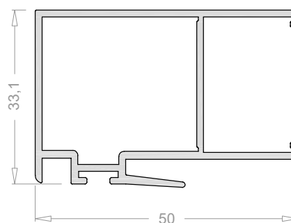
Hoja central 22 mm 5007
