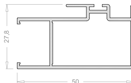
Hoja central 17 mm 6538
