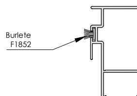
Hoja central 17 mm 6538
