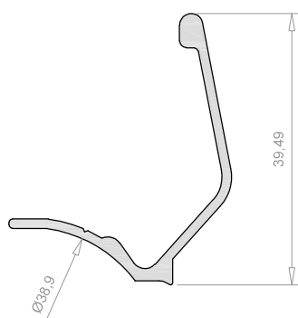
Remate Superior Marco 7603
