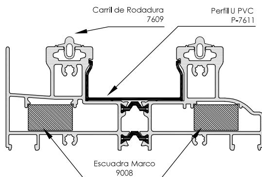
Marco Perimetral 7601
