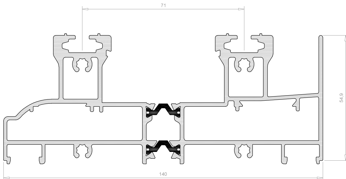
Marco Perimetral 7601
